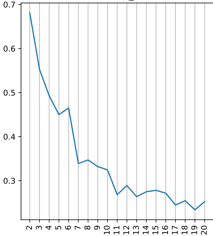
Silhouoette_score
